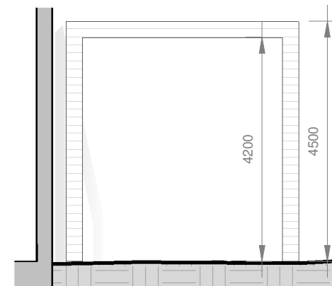
Portal - 02 - Front/Back Elevation 1 : 100
