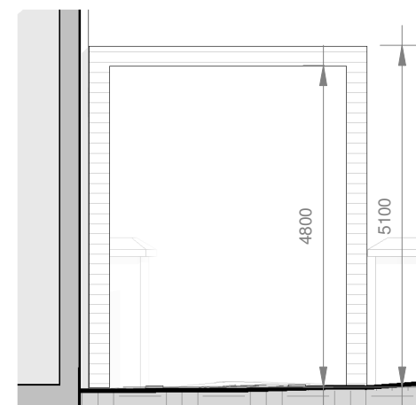
Portal - 03 - Front/Back 1 : 100
